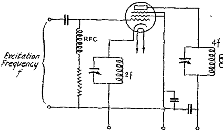
FIG. 1—THE FUNDAMENTAL CIRCUIT OF THE "DOUBLE-DOUBLER"
