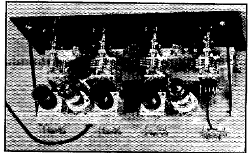
PLAN VIEW OF THE EXCITER UNIT SHOWING IN DETAIL THE ARRANGEMENT OF THE COMPONENTS
